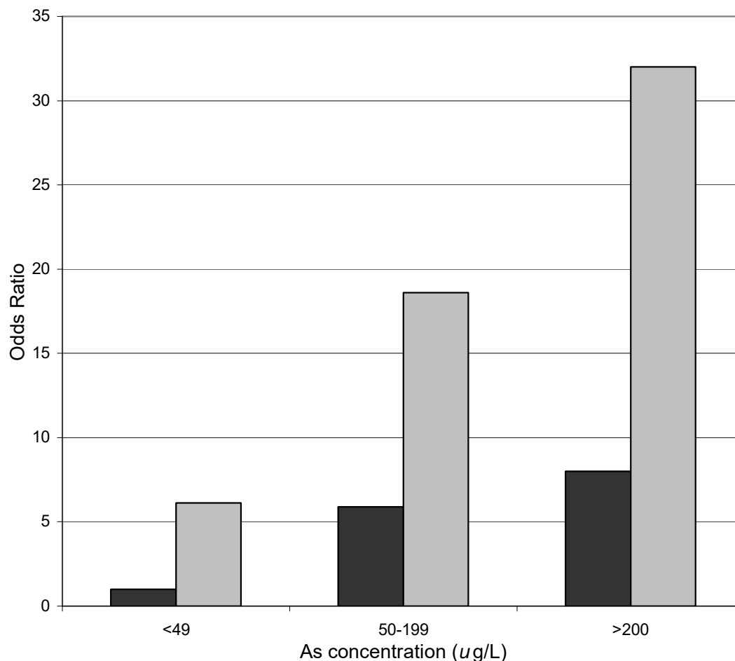
Figure 5: Lung Cancer Risk (OR) Associated with As Concentration in Drinking Water and Smoking (Ferrecio et al., 2000)
