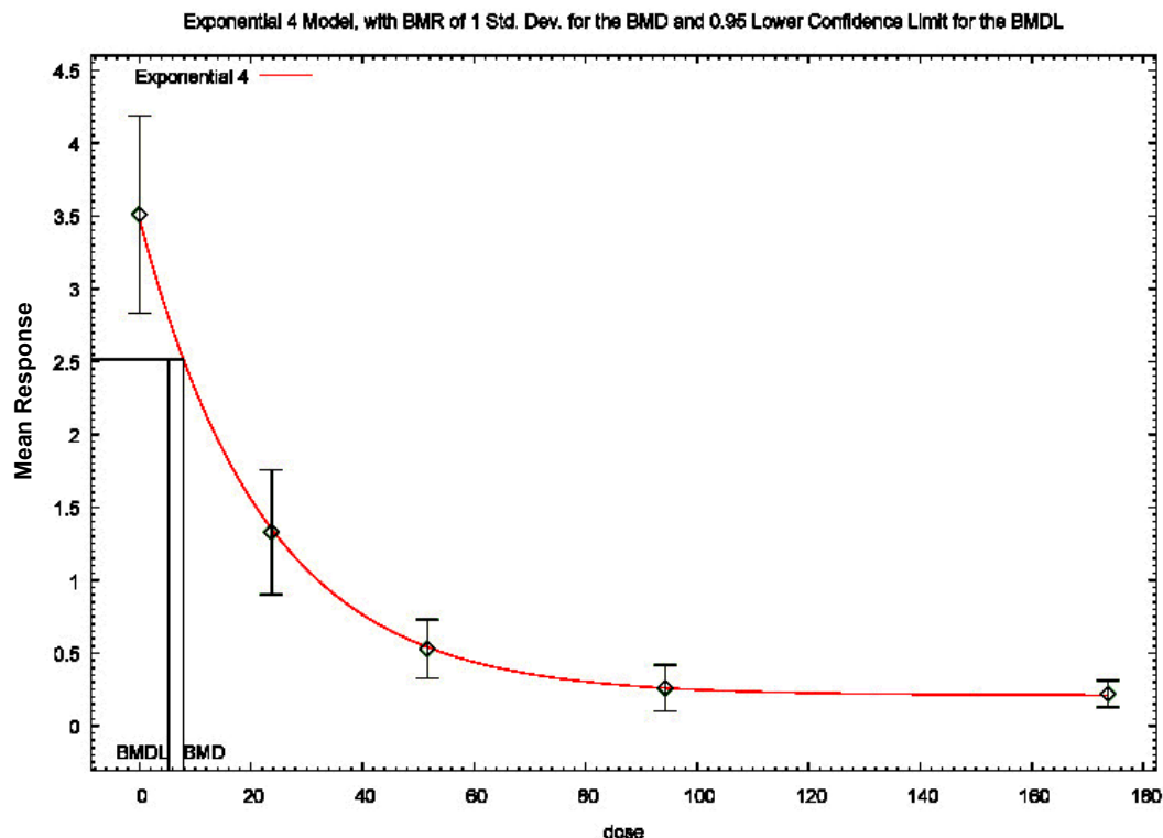
Figure A10.19. BMD modeling of decreased total T4 in male Sprague Dawley rats from NTP (2019b) (high dose excluded)
