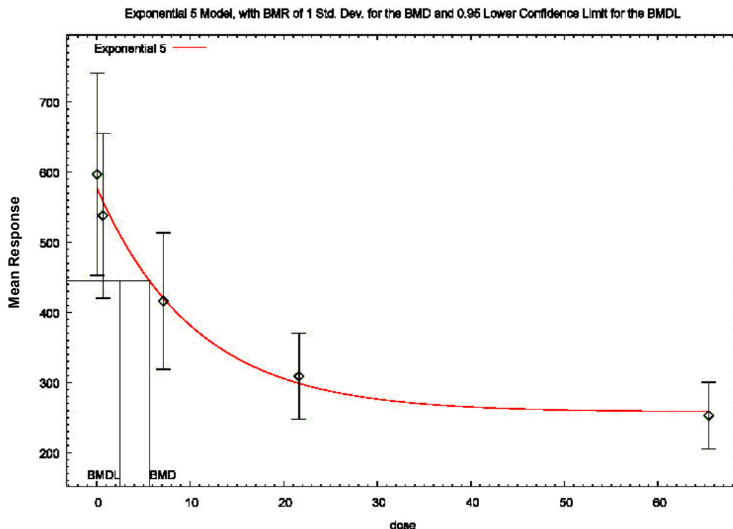
Figure A10.22. BMD modeling of decreased plaque forming cell response in male c57/BL6 mice from Dong et al. (2009) (BMR = 1 standard deviation)
