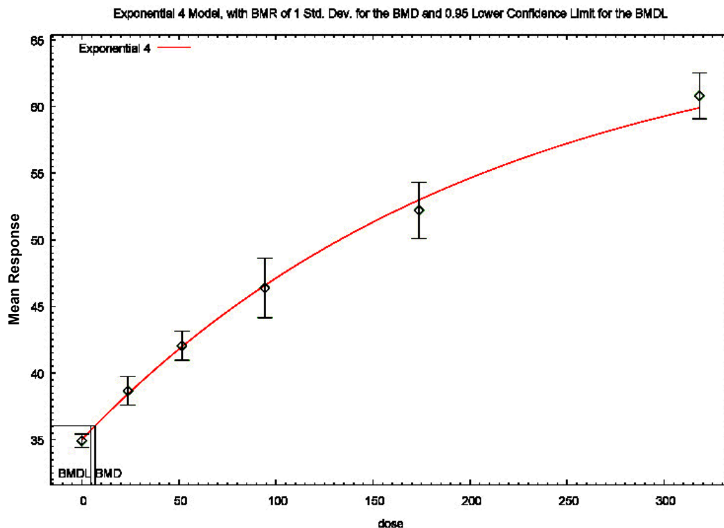
Figure A10.17. BMD modeling of increased relative liver weight in male Sprague Dawley rats from NTP (2019b)
