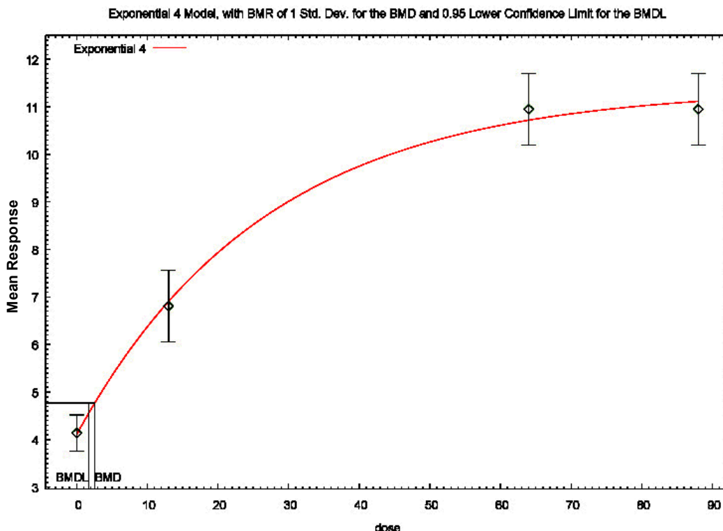
Figure A10.10. BMD modeling of increased relative liver weight in male BALB/c mice from Guo et al. (2019)
