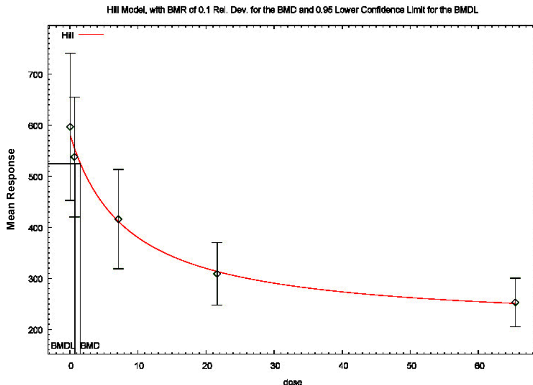
Figure A10.23. BMD modeling of decreased plaque forming cell response in male c57/BL6 mice from Dong et al. (2009) (BMR = 0.1 relative deviation)
