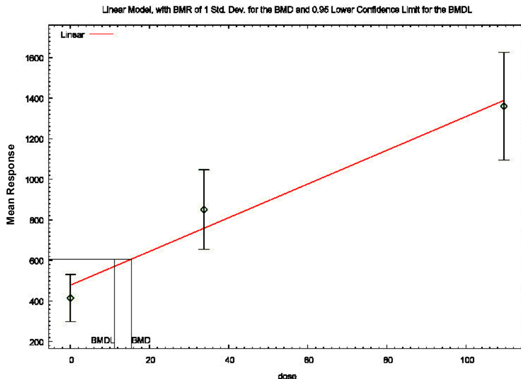
Figure A10.15. BMD modeling of increased liver triglycerides in female CD-1 mice from Lai et al. (2018)
