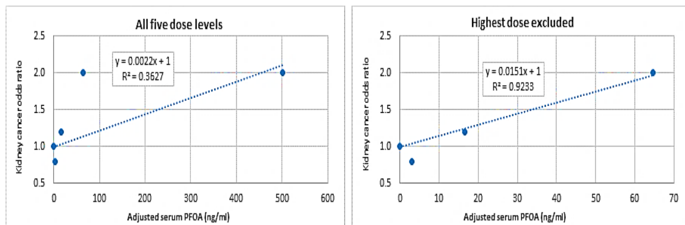
Figure 6.2.4. Simple linear regression analysis of serum PFOA and kidney cancer ORs from Vieira et al. (2013) with and without the highest exposure (dose) category
