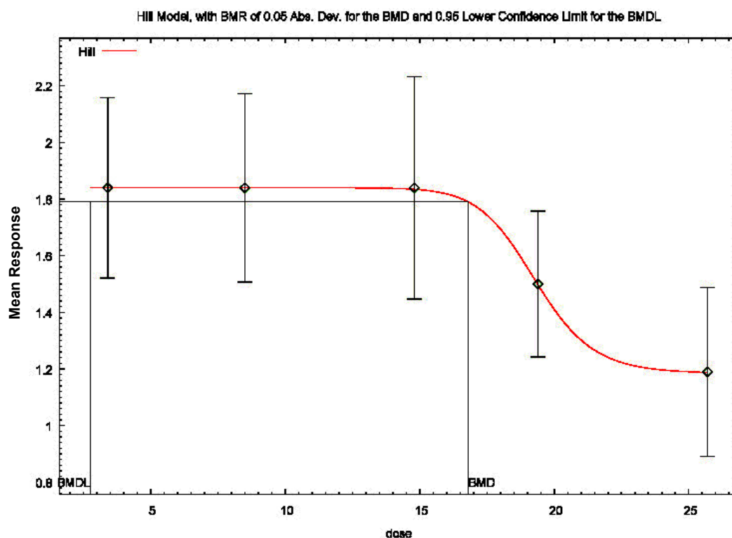
Figure A10.1. BMD modeling of decreased influenza (Hib) antibody levels in humans from Abraham et al. (2020)
