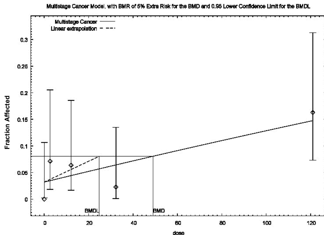
Figure A10.24. BMD modeling of hepatocellular tumor incidence in male Sprague Dawley rats from Butenhoff et al. (2012b)
