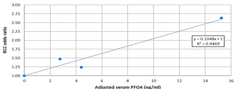
Figure 6.2.3. Simple linear regression analysis of serum PFOA and RCC ORs from Shearer et al. (2021)
