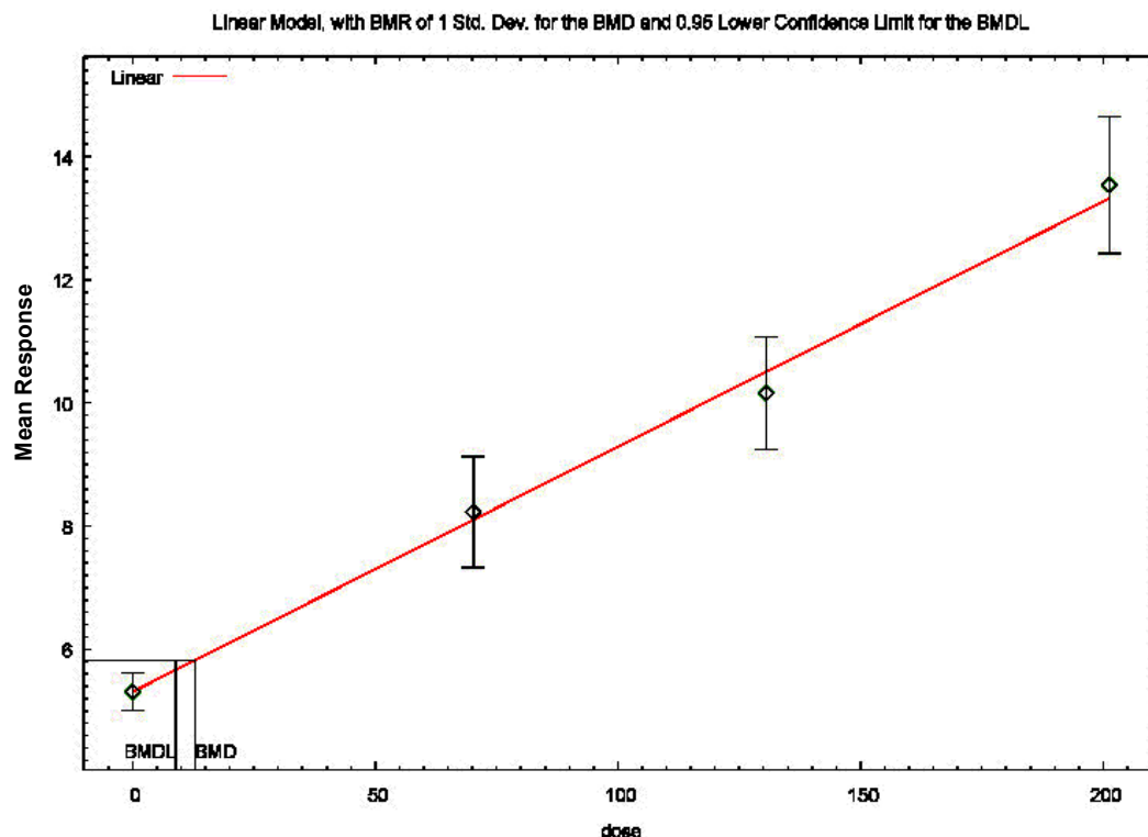
Figure A10.14. BMD modeling of increased relative liver weight in male C57BL/6 mice from Xing et al. (2016)
