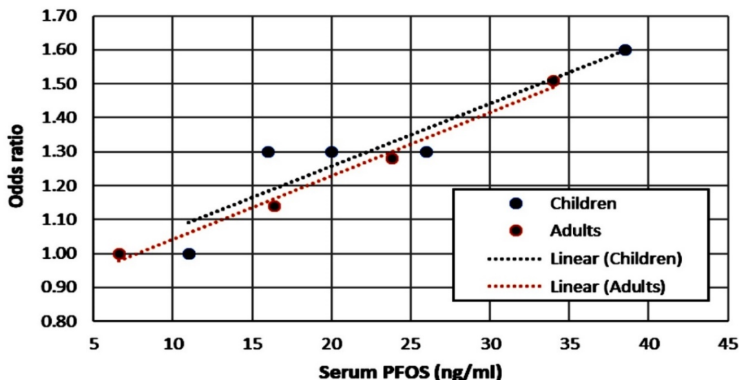
Figure 6.1.1. Odds ratios for elevated serum TC by quantiles of serum PFOS (ng/ml) in adults Steenland et al. (2009) and children Frisbee et al. (2009) from the C8 study area
