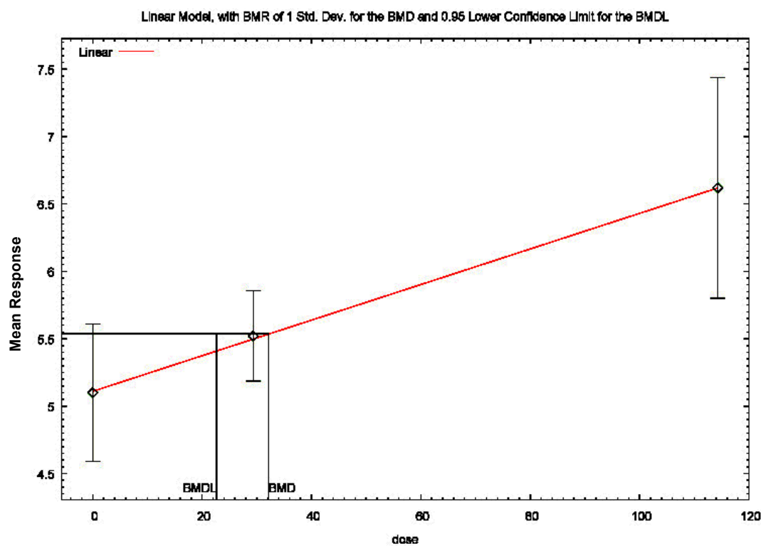
Figure A10.8. BMD modeling of increased relative liver weight weight in male BALB/c mice from Yu et al. (2016)
