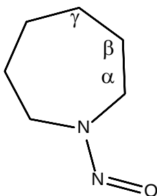
Figure 1. Structure of N-Nitrosohexamethyleneimine.
