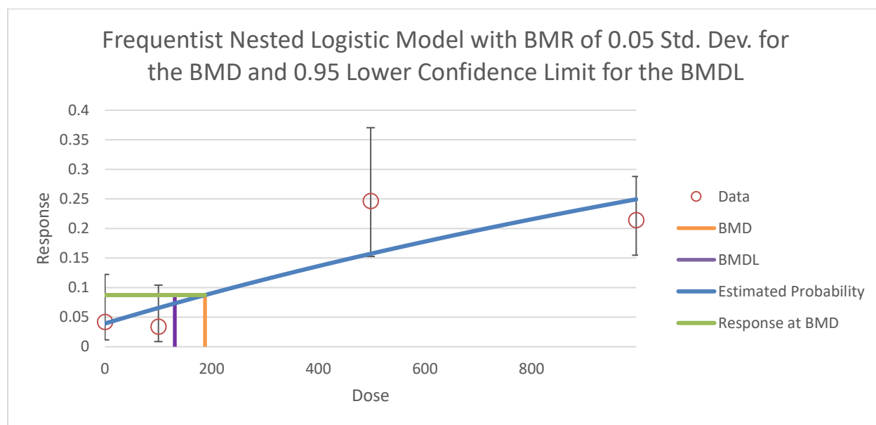
Figure 2. Nested logistic model fit to the skull ossification data in rat fetuses exposed to 1-BP during gestation (Huntingdon Life Sciences, 2001)
