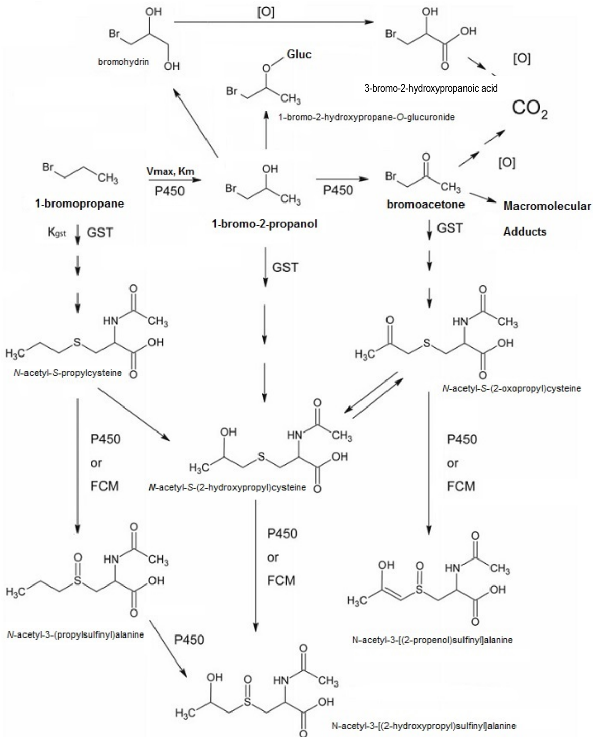
Figure 1. Metabolism of 1-BP in rodents: modified from Figure 2 of Garner et al. (2015). GST = glutathione-S-transferase; FCM = Flavin monooxygenase; V_{max} = maximal velocity; K_m = Michaelis Constant; K_{gst} = proportionality constant for linear pathway metabolized by glutathione transferase; \rightleftharpoons multiple steps of reaction; [O] = unspecified oxidation step
