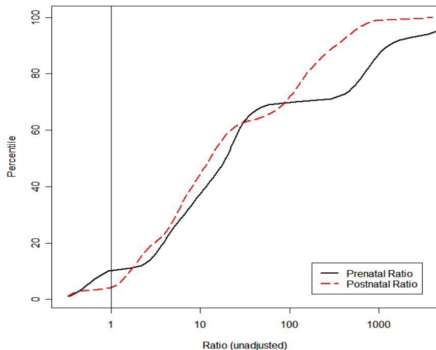
Figure 21. ENU Prenatal and Postnatal LP j Ratio Cumulative Distribution Functions – Equal Weighting of Potency Distributions
