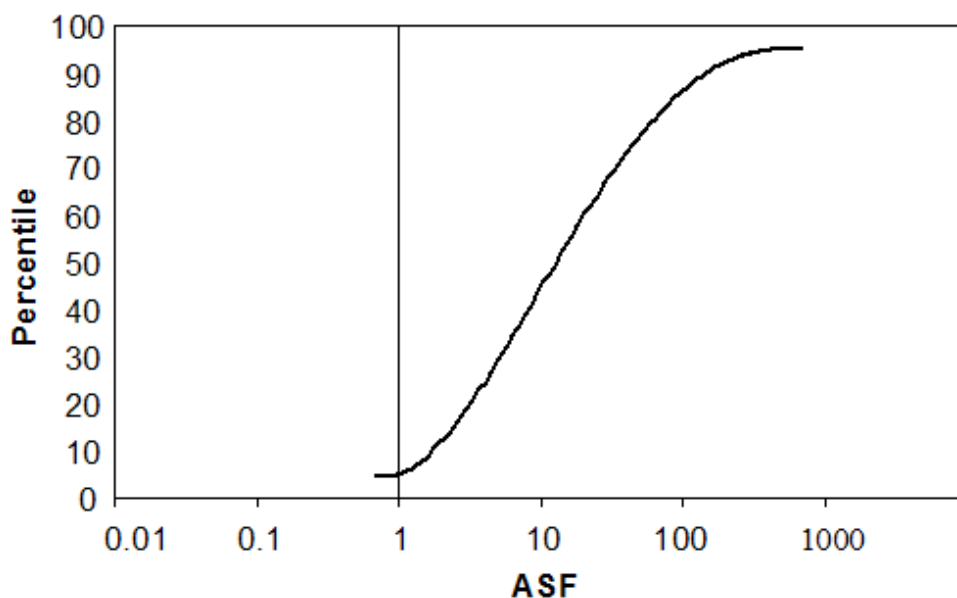
Figure 13. Postnatal ASF Mixture Distribution
