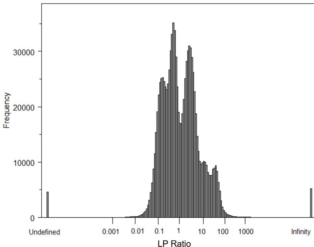
Figure C-1a. Prenatal LP Ratio Mixture Frequency Distribution – Equally Weighted Chemicals, Equally Weighted Studies (Method 1, presented in the main text)
