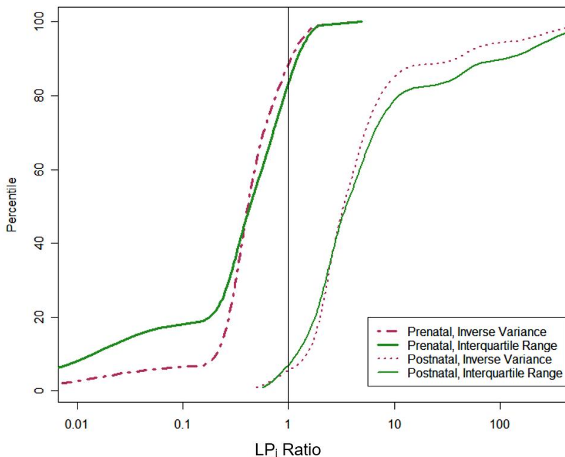
Figure D-2. Methods 2a and 2b DEN Prenatal and Postnatal LP j Ratio Cumulative Distribution Functions – Inverse-Variance and Interquartile Weighting of Potency Distributions
