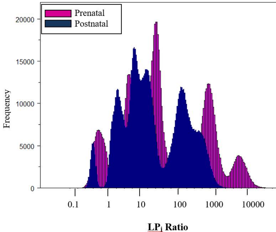
Figure E-1. Method 1 ENU Prenatal and Postnatal LP j Ratio Frequency Distributions – Equal Weighting of Potency Distributions
