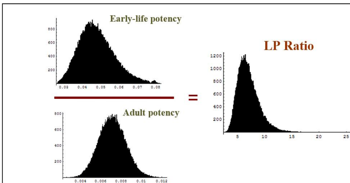
Figure 5. Lifestage Potency (LP) Ratio Distribution
