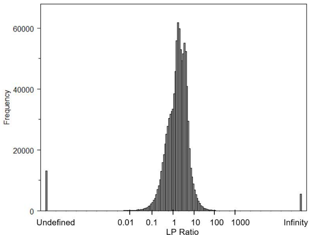
Figure C-3a. Juvenile LP Ratio Mixture Frequency Distribution – Equally Weighted Chemicals, Equally Weighted Studies (Method 1, presented in the main text)
