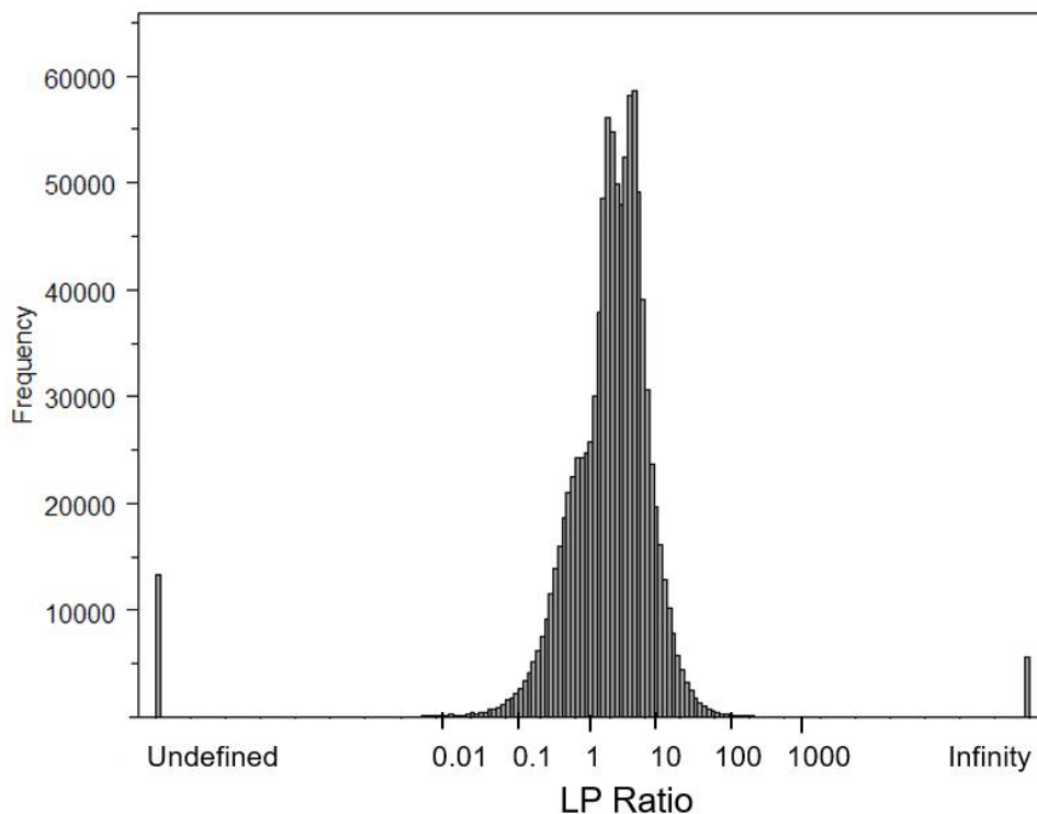
Figure C-3c. Juvenile LP Ratio Mixture Frequency Distribution - Equally Weighted Chemicals, Single Study Represents Each Chemical (Method 3)
