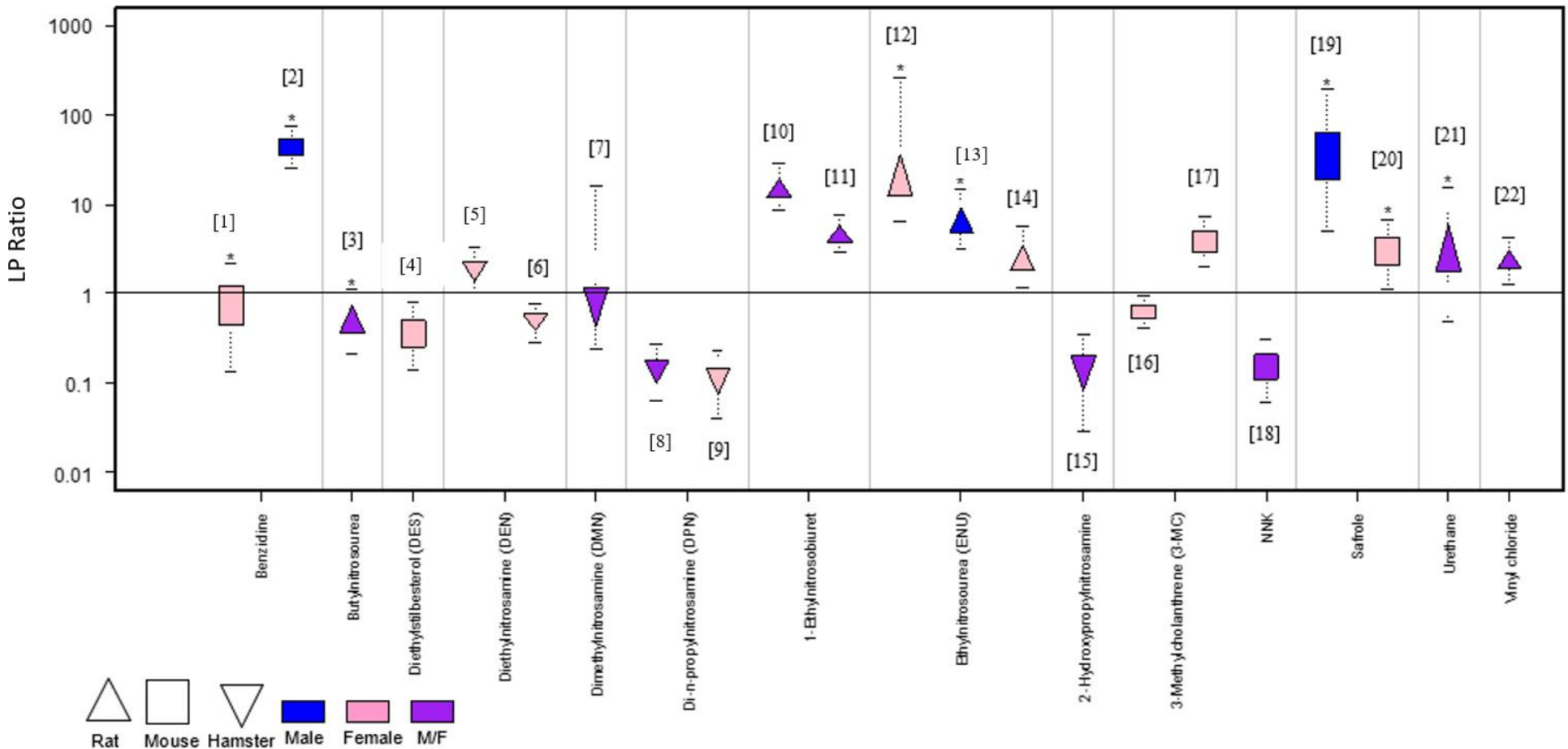
Figure 6. Prenatal LP Ratio Distributions
