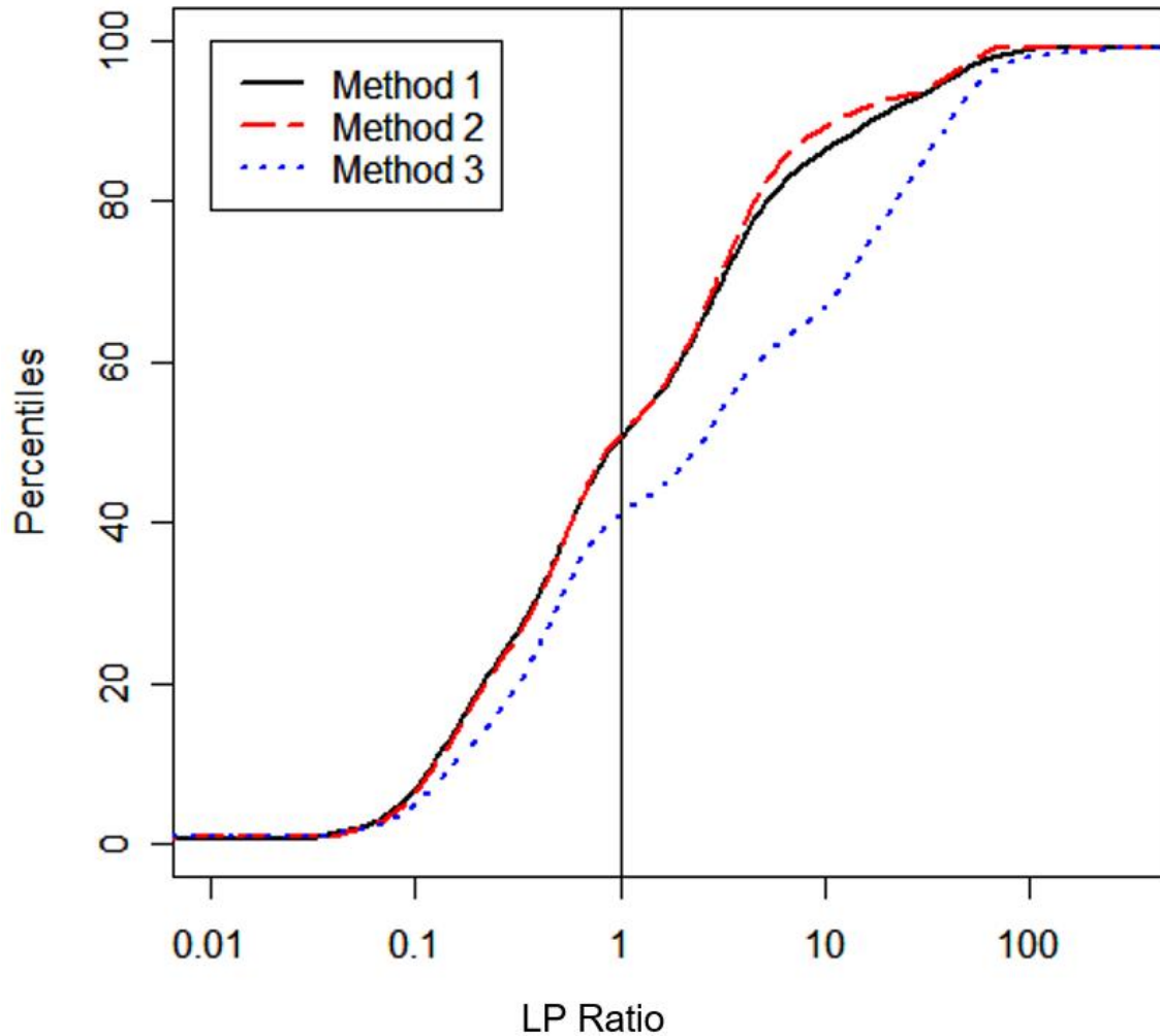
Figure 7. Prenatal LP Ratio Mixture Cumulative Distribution Functions
