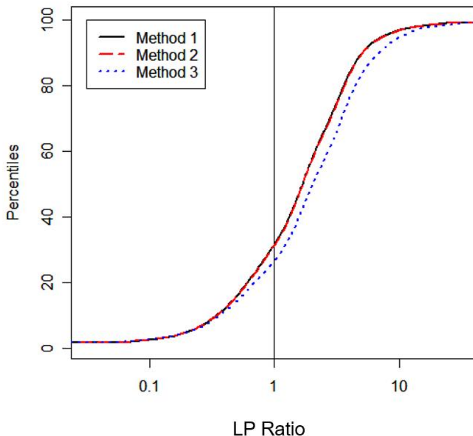
Figure 15. Juvenile LP Ratio Mixture Cumulative Distribution Functions
