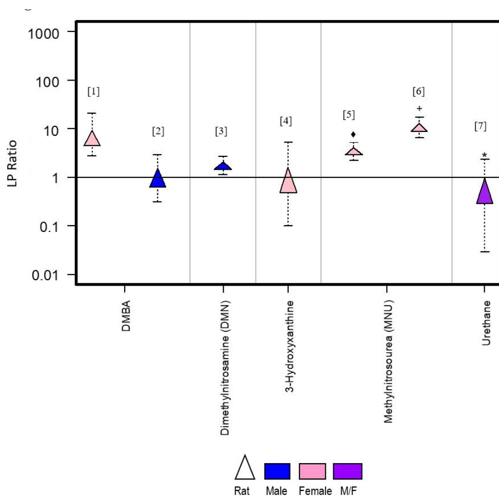
Figure 14. Juvenile LP Ratio Distributions
