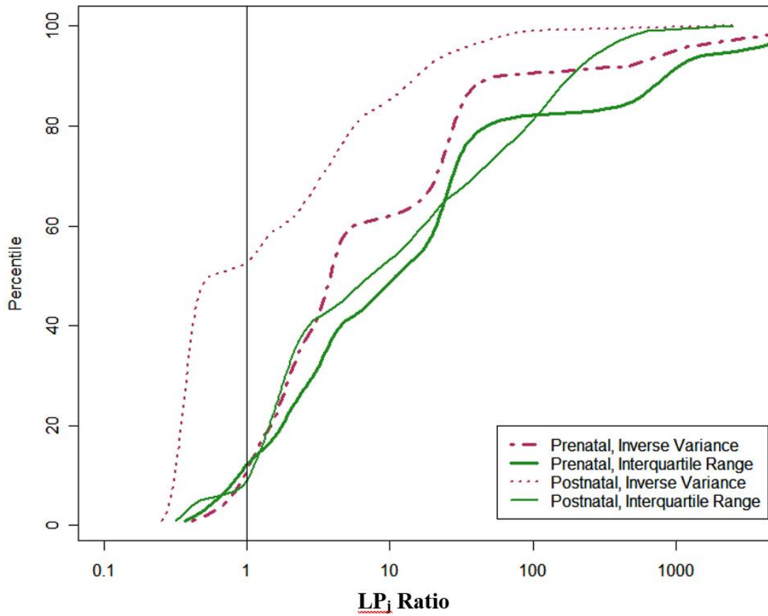
Figure E-2. Methods 2a and 2b ENU Prenatal and Postnatal LP_j Ratio Cumulative Distribution Functions – Inverse-Variance and Interquartile Weighting of Potency Distributions
