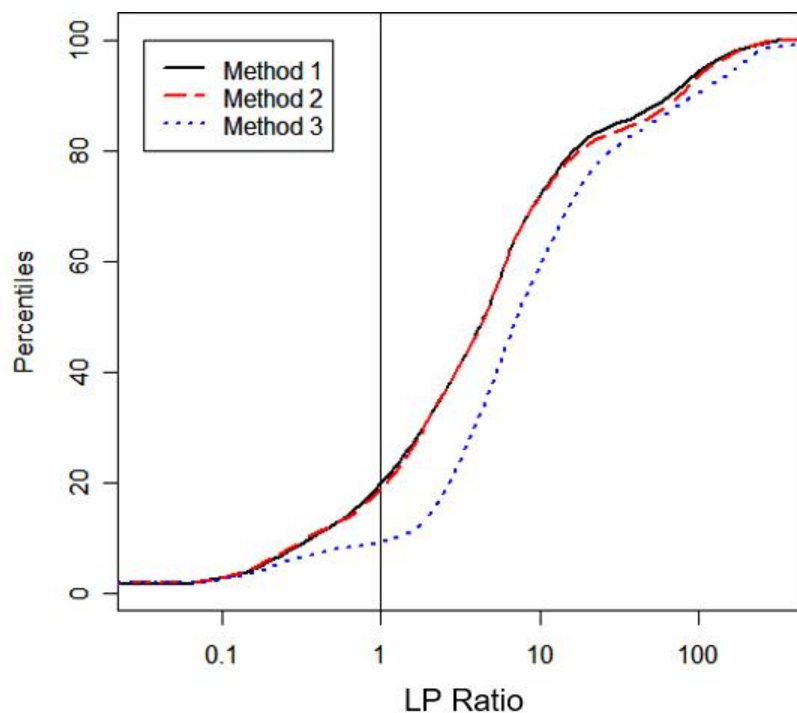
Figure 11. Postnatal LP Ratio Mixture Cumulative Distribution Functions
