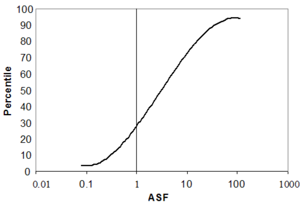
Figure 9. Prenatal ASF Mixture Distribution
