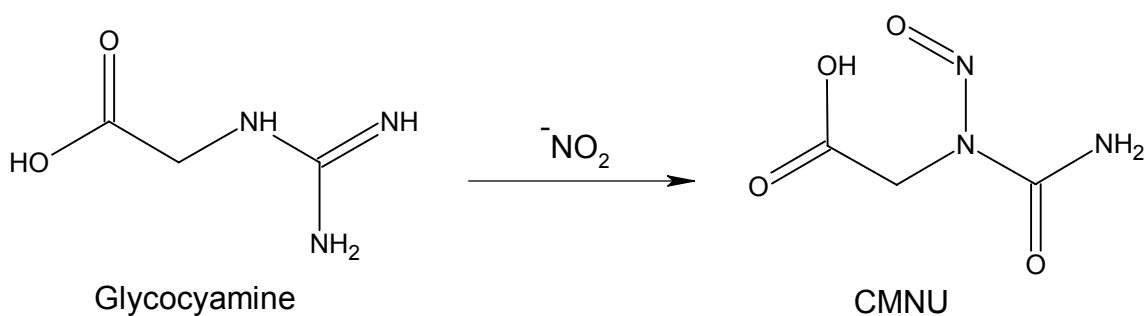
Figure 2. Formation of CMNU from glycoxyamine and nitrite
