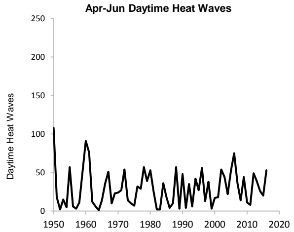
Figure 3. Statewide trends in daytime heat waves and extreme heat days
